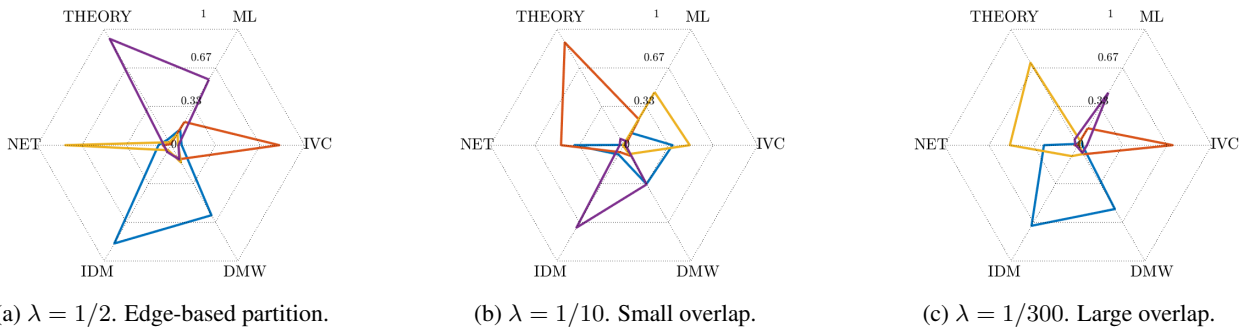
1206 Figure 9: Partitioning the DBLP co-authorship graph in four communities. The edge based partitions sharply correlate to 1207 specific computing areas. As the overlap increases communities become more rounded, losing their clear definition. 1208 1209
