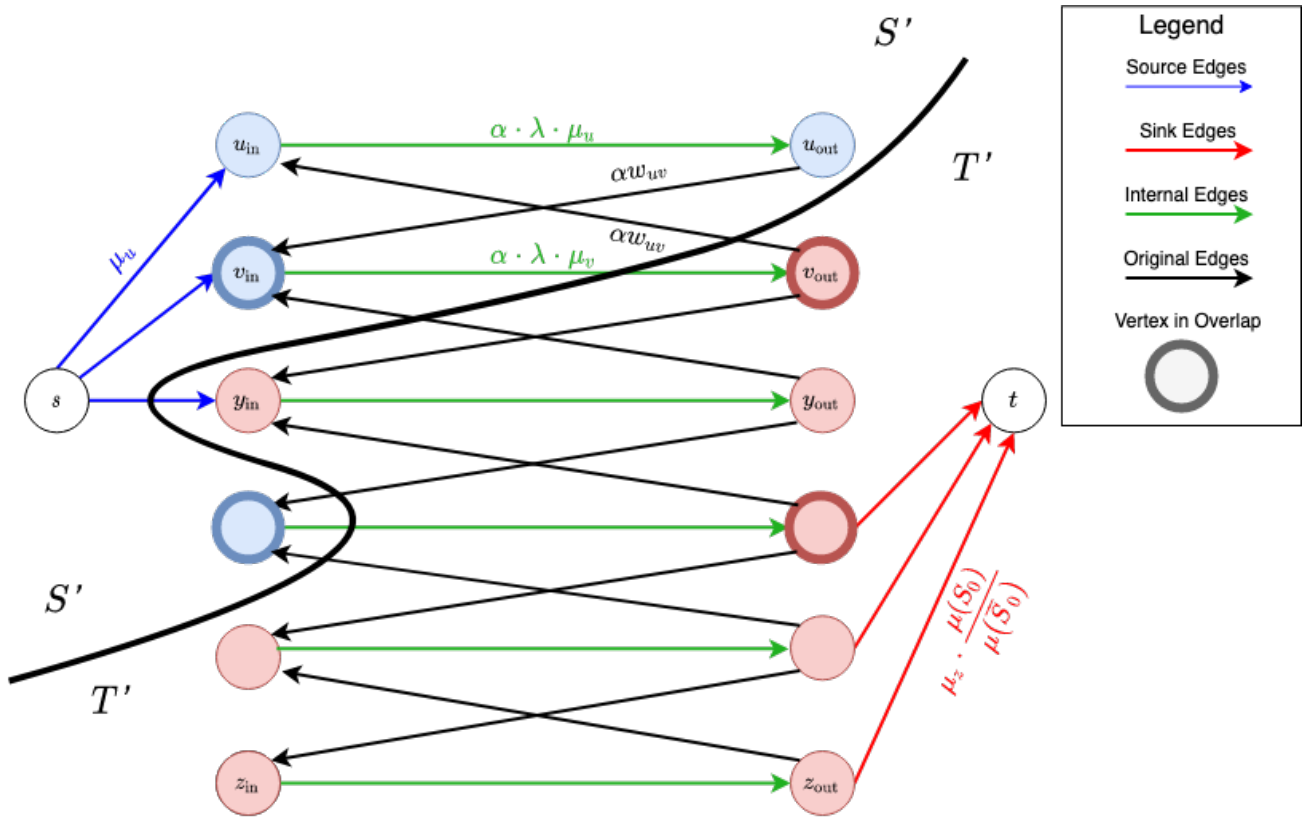
Figure 4: A valid s - t mincut (S', T') of G_\alpha , together with the corresponding overlapping partition.
