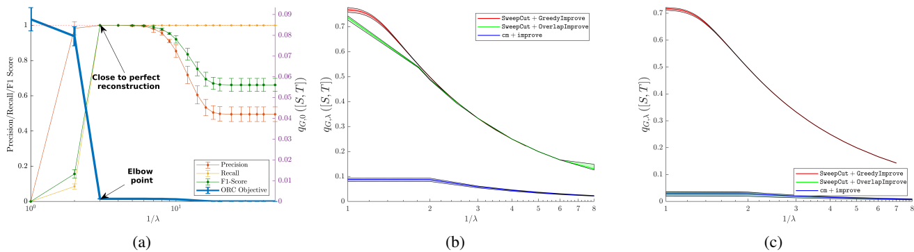
Figure 2: (a) Statistical performance of cm+improve in the recovery of the ground-truth overlap C on 5 samples on balanced OSBM with parameters (|C|, p, \epsilon) = (100, 4, 0.05) . (b) Comparison on balanced OSBM with parameters (|C|, p, q, \epsilon) = (10, 4, 4, \epsilon = 0.05) . (c) Comparison on balanced OSBM with parameters (|C|, p, q, \epsilon) = (10, 4, 4, \epsilon = 0.05) .
