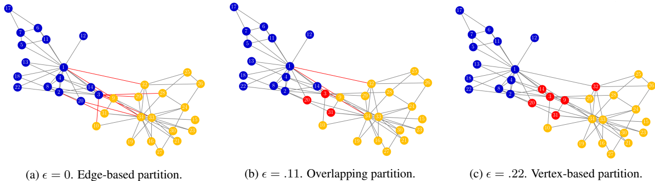
Figure 1: Visualizations of overlapping solutions to \epsilon -ORC for different values of \epsilon \in [0, 1] on the Karate graph (Zachary, 1977), with \mu set to the degree measure. Partition sides are yellow and blue. Overlap is red. Cut edges are also red. Solutions were computed using our algorithm cm+improve .
