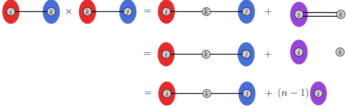
Figure 2.6: (First equality) The left side sums over all i, j, k . The first term on the right side has terms where i \neq j , and the second term has terms where i = j (purple denotes U_\alpha \cap V_\alpha ). The second term is an improper shape, since when i = j , both edges become \{i, k\} . (Second equality) Since A has Boolean entries, linearize A_{i,k}^2 = 1 . (Third equality) The isolated vertex scales the matrix by n - 1 .
