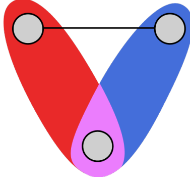
Figure 2.4: The purple vertex lies in U_\alpha \cap V_\alpha . For each choice of a label k for the purple vertex, for i, j \in [n] , the ((i, k), (j, k)) entries of the graph matrix are essentially a copy of the one-edge shape with U_\alpha \cap V_\alpha deleted. The ((i, k), (j, k)) entry is \chi_{\{i, j\}}(X) if i, j, k are distinct and 0 otherwise.
