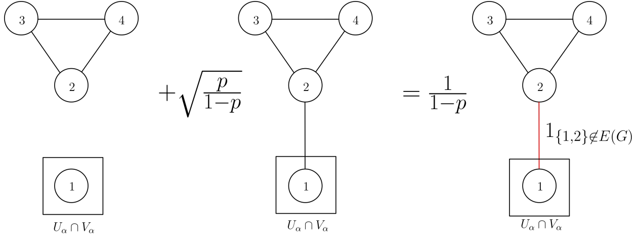
Figure 6.3: The two ribbons on the left side can be added together to get a multiple of the indicator function for the edge \{1,2\} , which is the red edge on the right. However, the leftmost ribbon does not appear due to the connected truncation.
