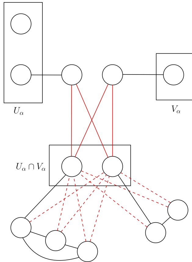
Figure 6.4: Example of a permissible shape. The solid red edges are independent set indicators. The dashed red edges represent two quasi-missing edge indicators between U_\alpha \cap V_\alpha and the two “floating” connected components of V(\alpha) \setminus (U_\alpha \cap V_\alpha) . Not shown are missing edge indicators between all pairs of vertices in U_\alpha and all pairs of vertices in V_\alpha .
