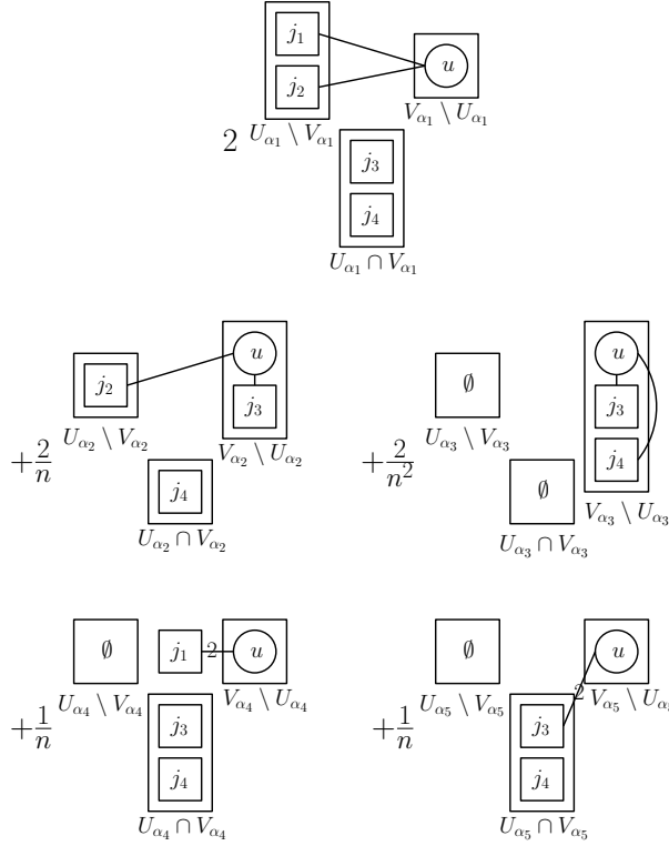
Figure 4.8: The five shapes that make up L_4 .
