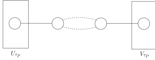
Figure 6.2: The shape from Fig. 6.1 after contracting edge pairs that have been charged to isolated vertices.
