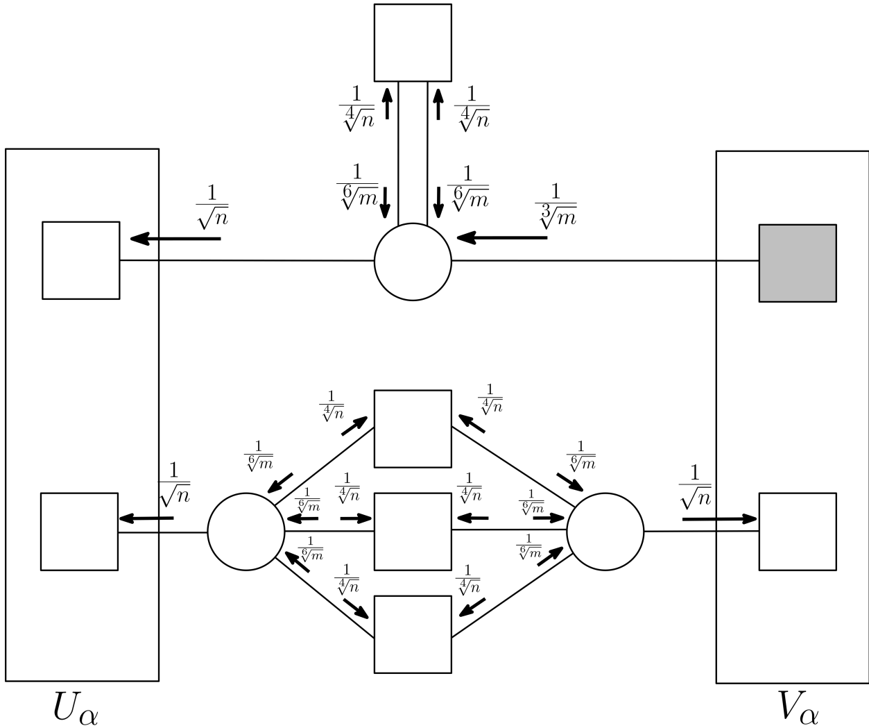
Figure 4.6: Allocation of \frac{1}{\sqrt{n}} from each edge to vertices. S consists of the gray square. Observe that every circle receives a factor of at least \frac{1}{\sqrt{m}} and every square not in S receives a factor of at least \frac{1}{\sqrt{n}} .
